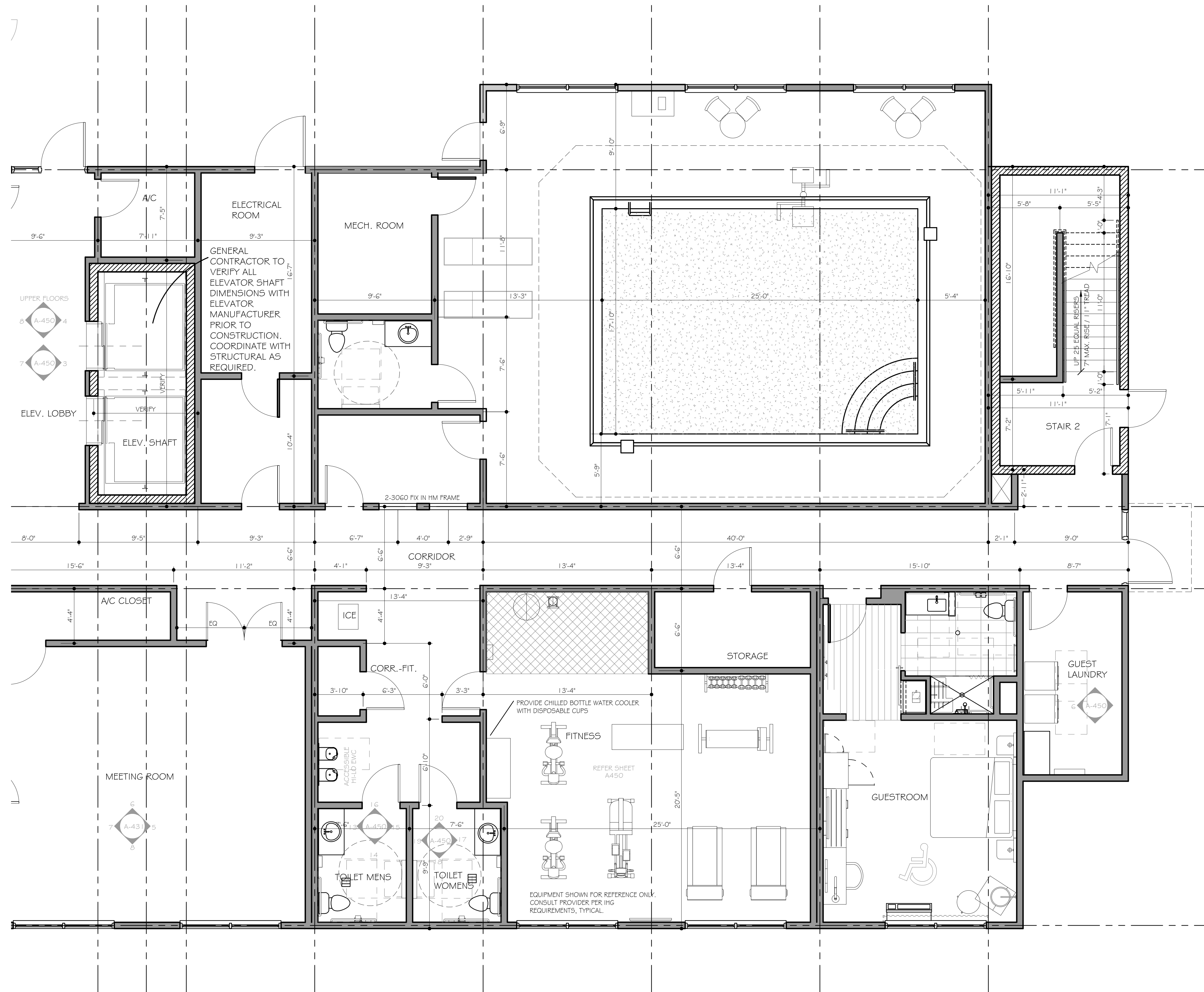
1 ENLARGED PARTIAL FIRST FLOOR PLAN SCALE: 1/4" = 1'-0"
