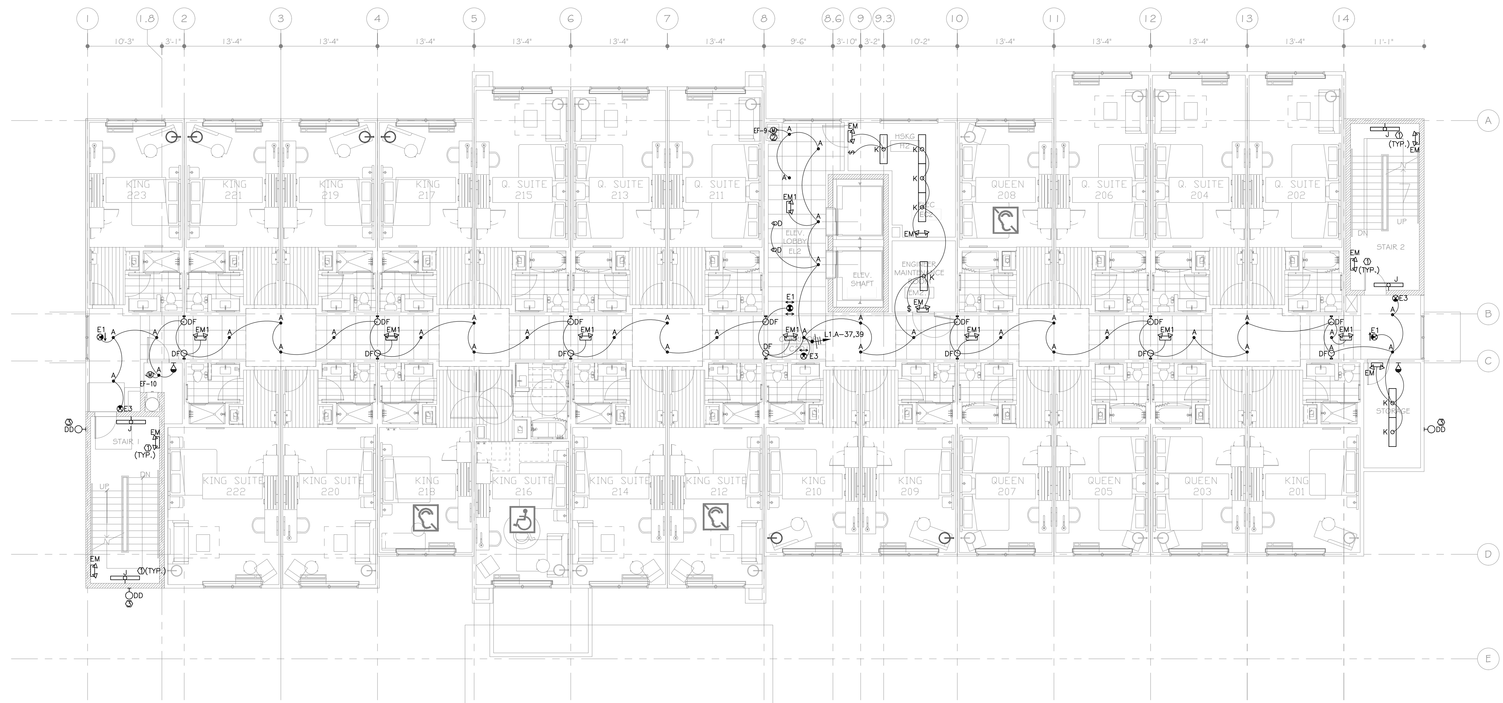
1 LIGHTING SECOND FLOOR PLAN SCALE: 1/8"=1'-0"
