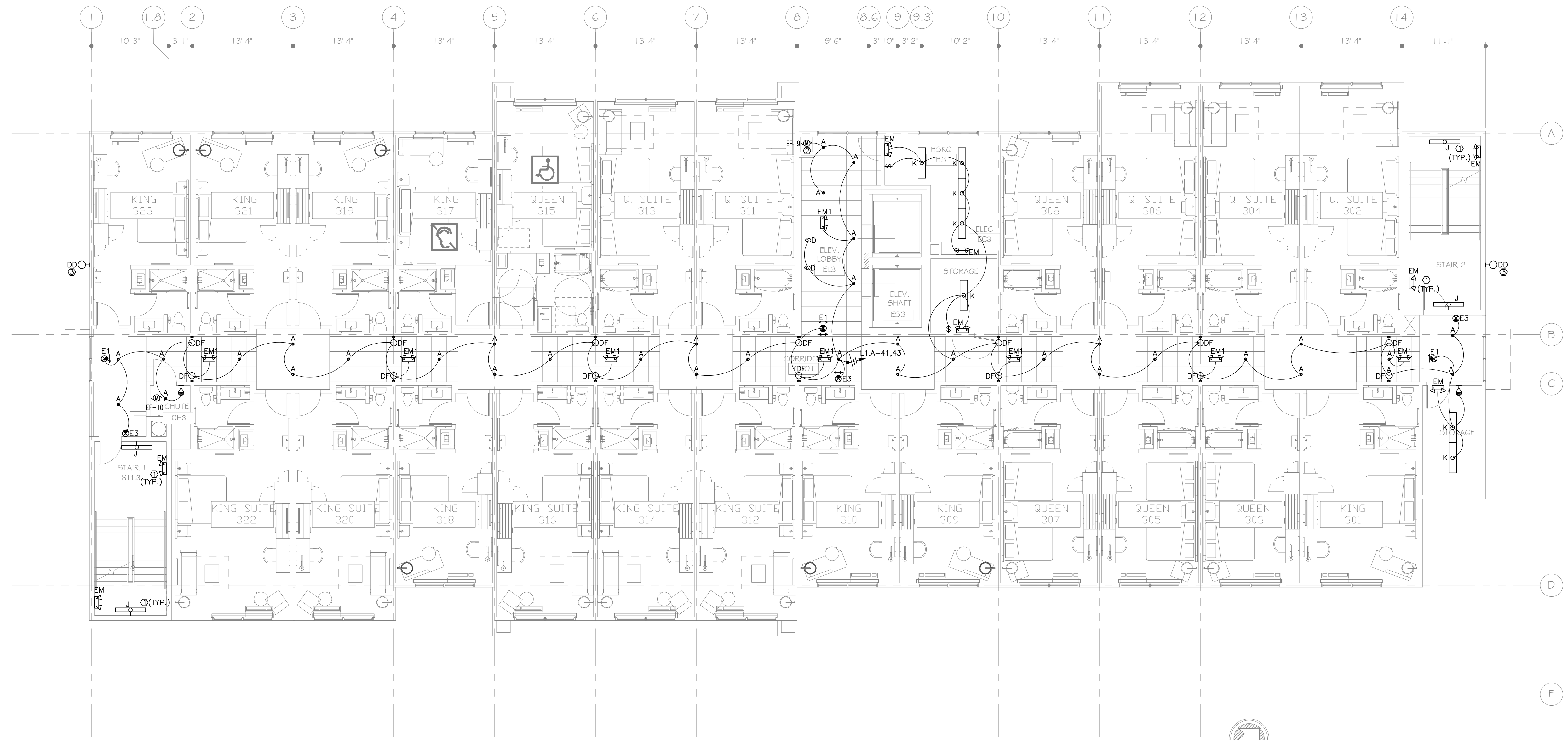
1 LIGHTING THIRD FLOOR PLAN SCALE: 1/8"=1'-0"
