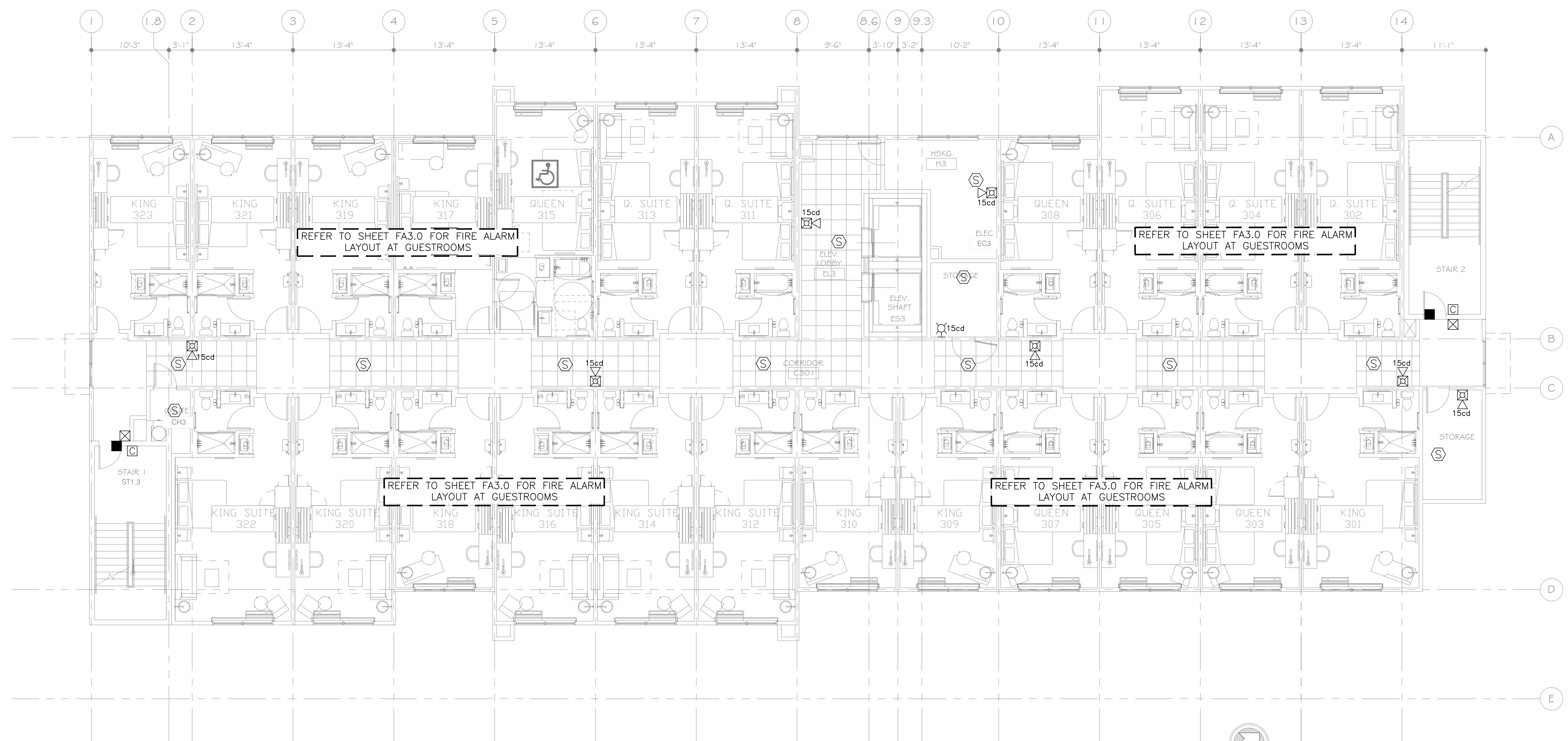
1 FIRE ALARM THIRD FLOOR PLAN SCALE: 1/8"=1'-0"
