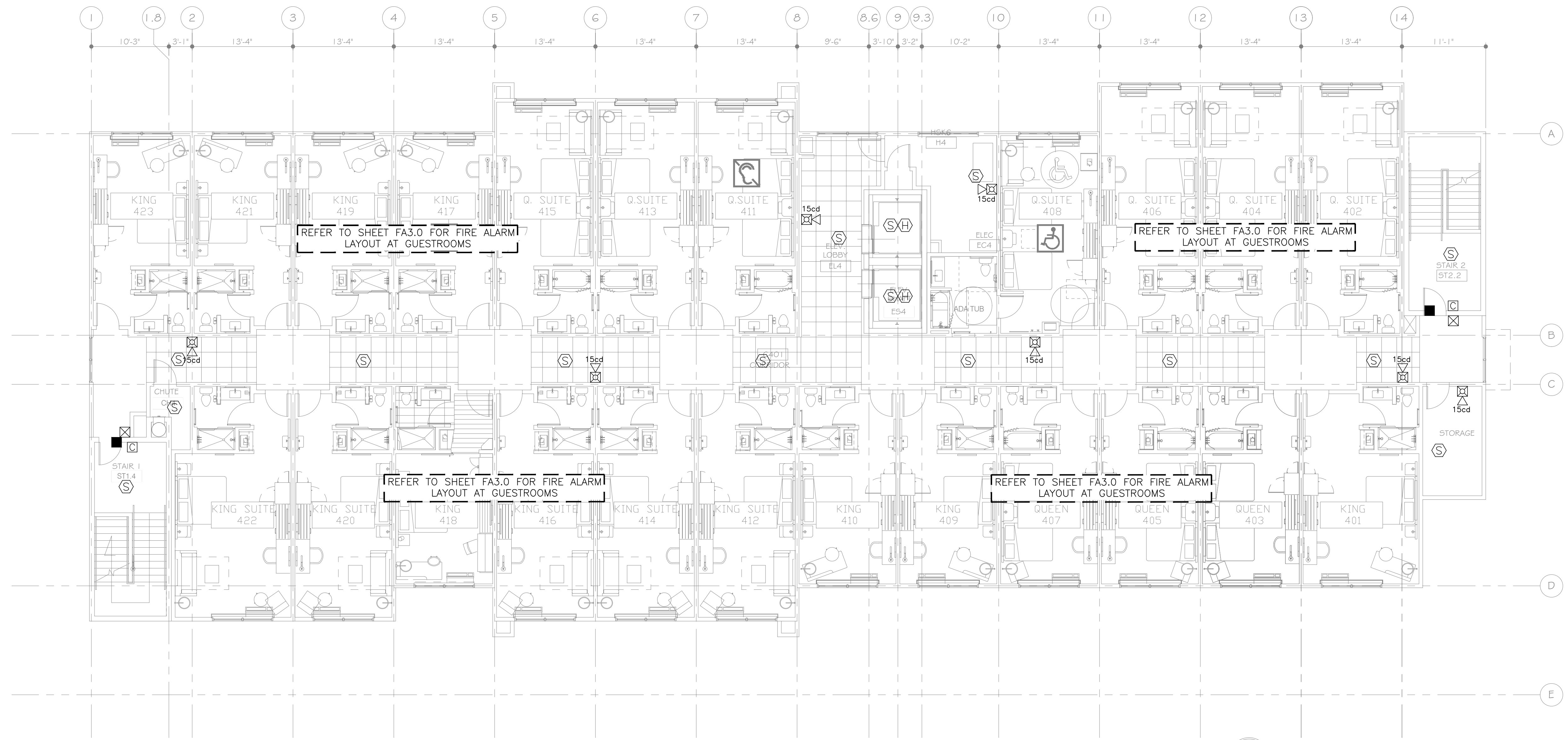
1 FIRE ALARM FOURTH FLOOR PLAN SCALE: 1/8"=1'-0"
