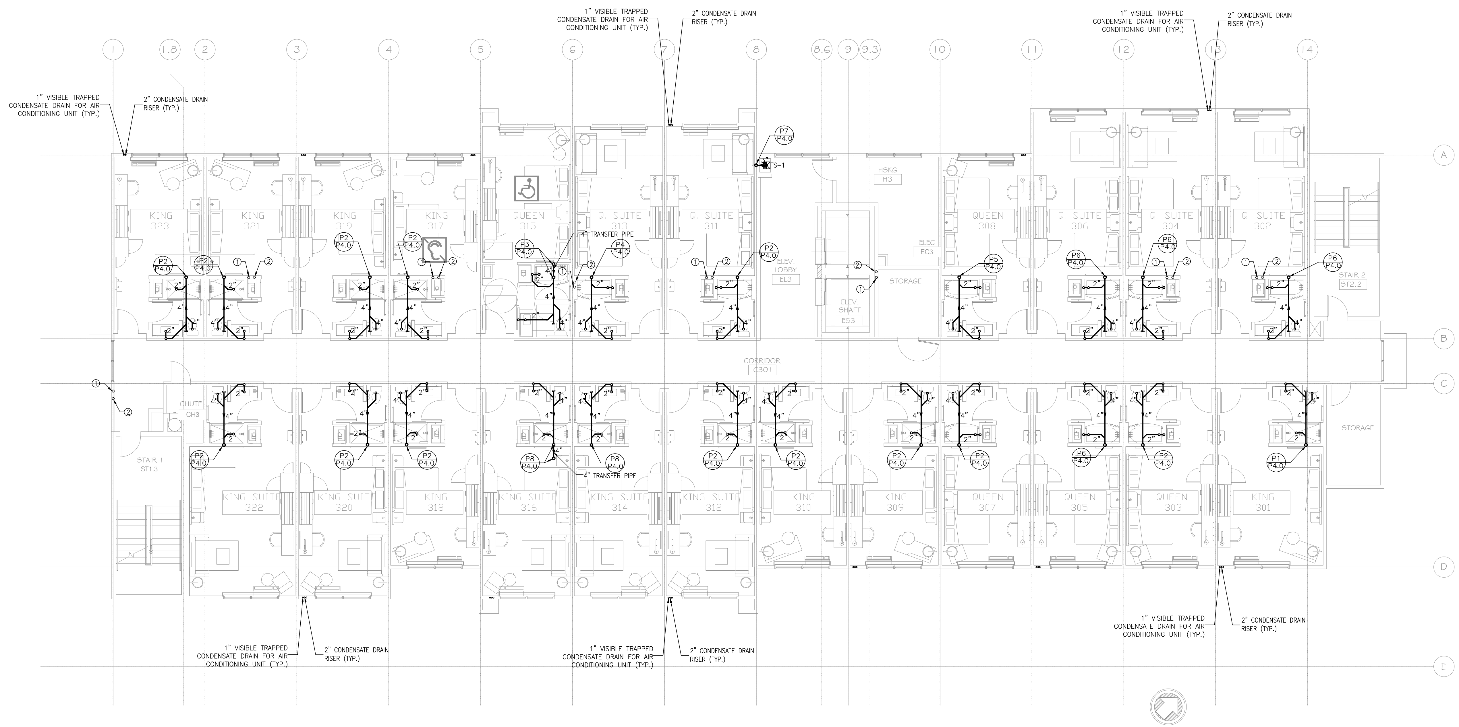
1 SANITARY SEWER THIRD FLOOR PLAN SCALE: 1/8"=1'-0"
