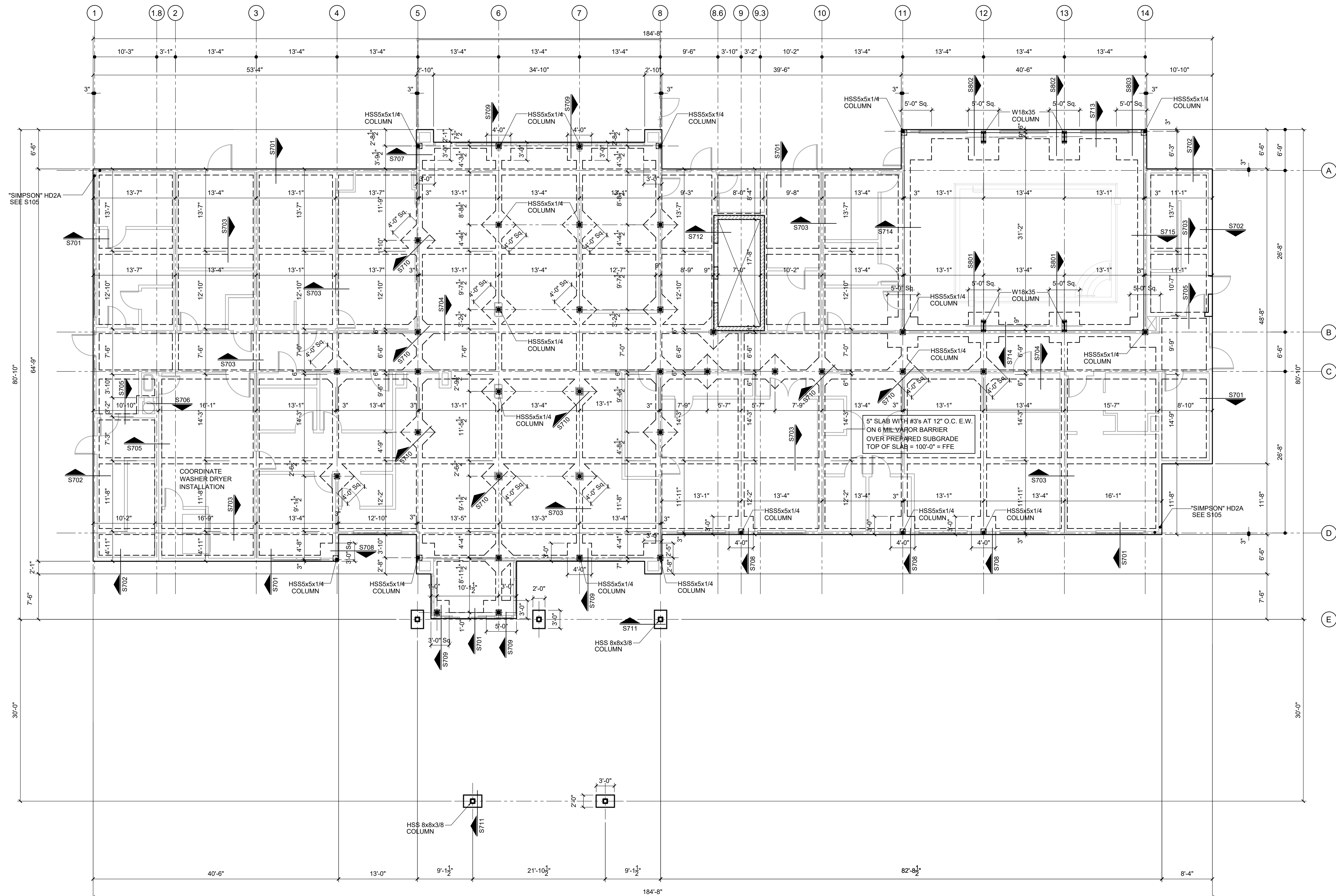
S201 FOUNDATION PLAN SCALE: 1/8" = 1'-0" NOTE: VERIFY ALL ASPECTS OF THE ELEVATOR WITH SELECTED MANUFACTURE BEFORE CASTING ELEVATOR PIT, INCLUDING DEPTH AND SIZE OF OPENING, ETC.
