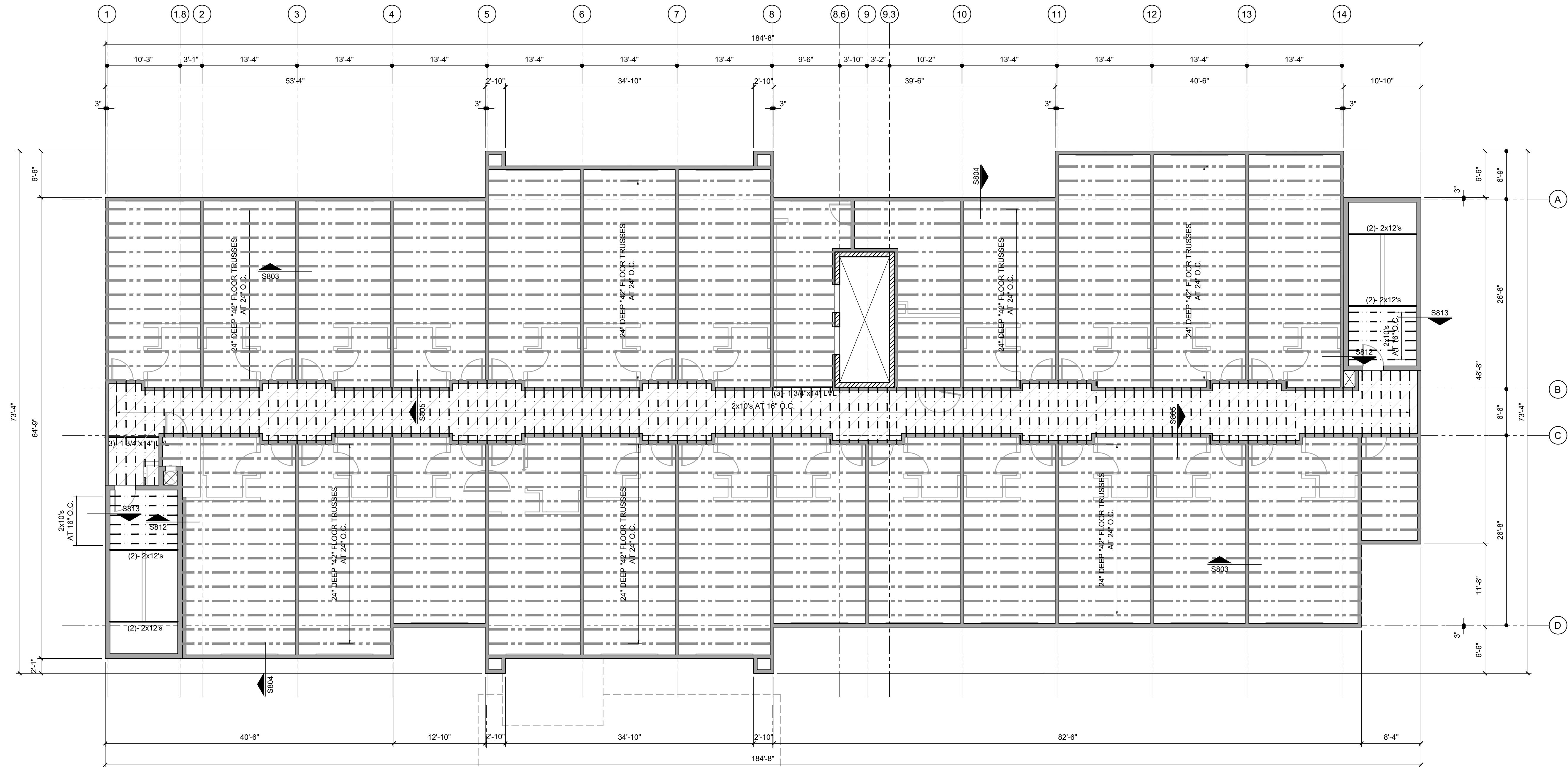
S401 THIRD FLOOR FRAMING PLAN SCALE: 1/8" = 1'-0"
