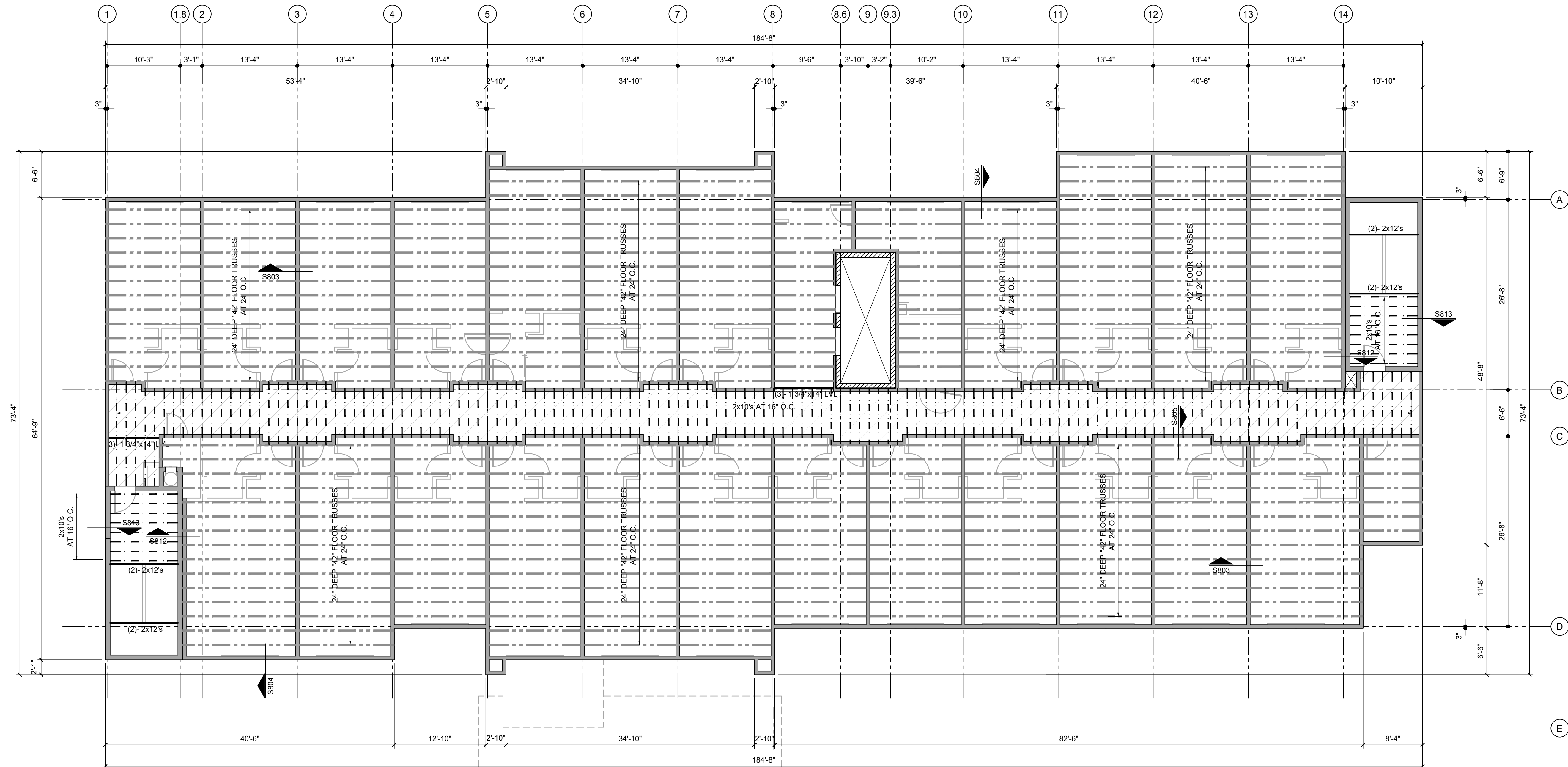
S501 FOURTH FLOOR FRAMING PLAN SCALE: 1/8" = 1'-0"
